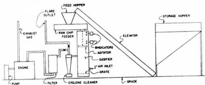
Fig. 2. Downdraft gasifier system.
