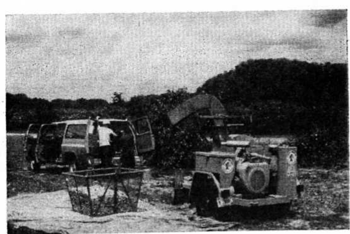
Fig. 1. Flywheel type chipper and collecting system.
