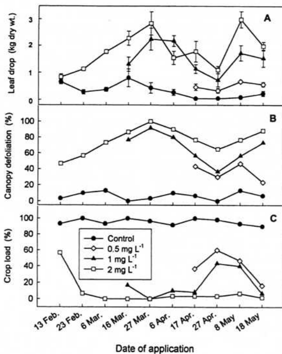
Fig. 4. Effect of application time and concentration of metsulfuron-methyl on (A) leaf drop after 21 d, and on (B) estimated canopy defoliation and (C) crop load (young fruit) after 60 d. Bars in (A) indicate se.
