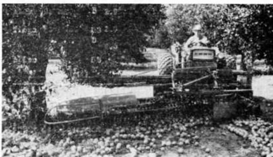
Fig. 4.—Windrowing rake with side-shift control.
