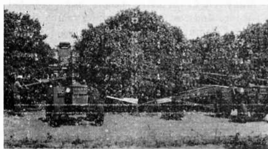
Fig. 1.—Tree shaker-catch frame harvest system.
